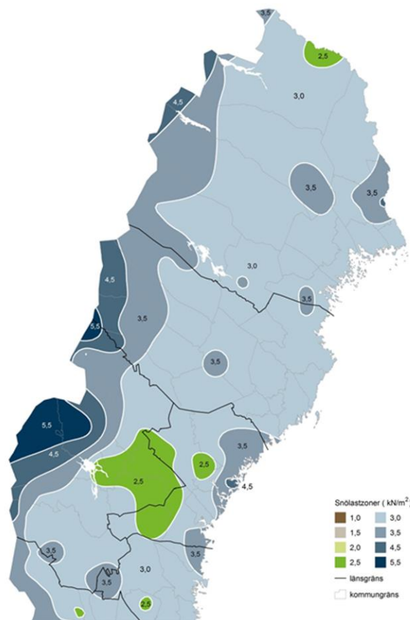
Figure 56: Snow load zones north of 60°N in Sweden, where it is most important to consider snow loads when constructing a building. The numbers given in this map range between 2.5 kN/m² and 5.5 kN/m². They can be used to dimension for extra roof loads due to snow when constructing a building in the regions described in the Swedish application of Eurocode 1 [171].
