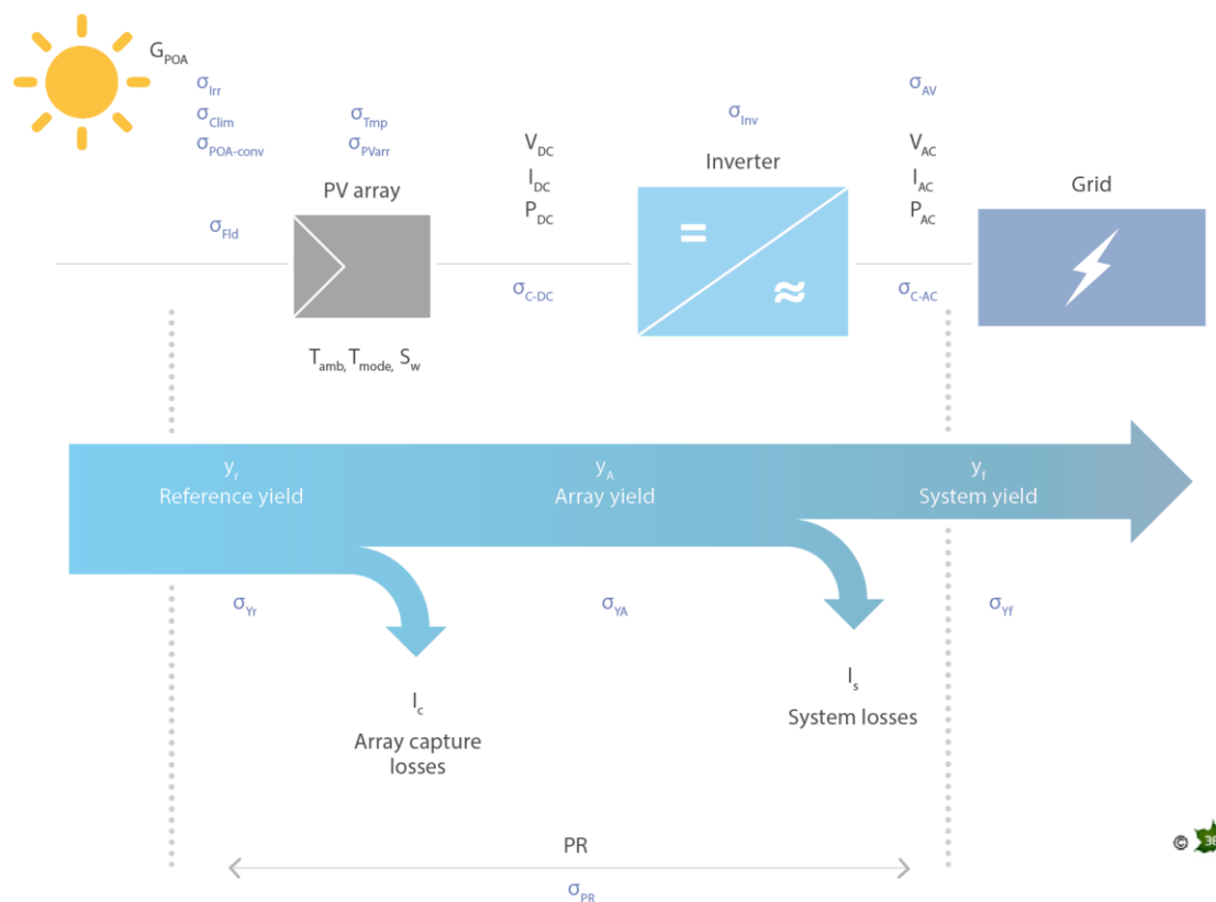
Figure 3: Energy flow diagram in a grid-connected photovoltaic system (source: 3E [19]).
