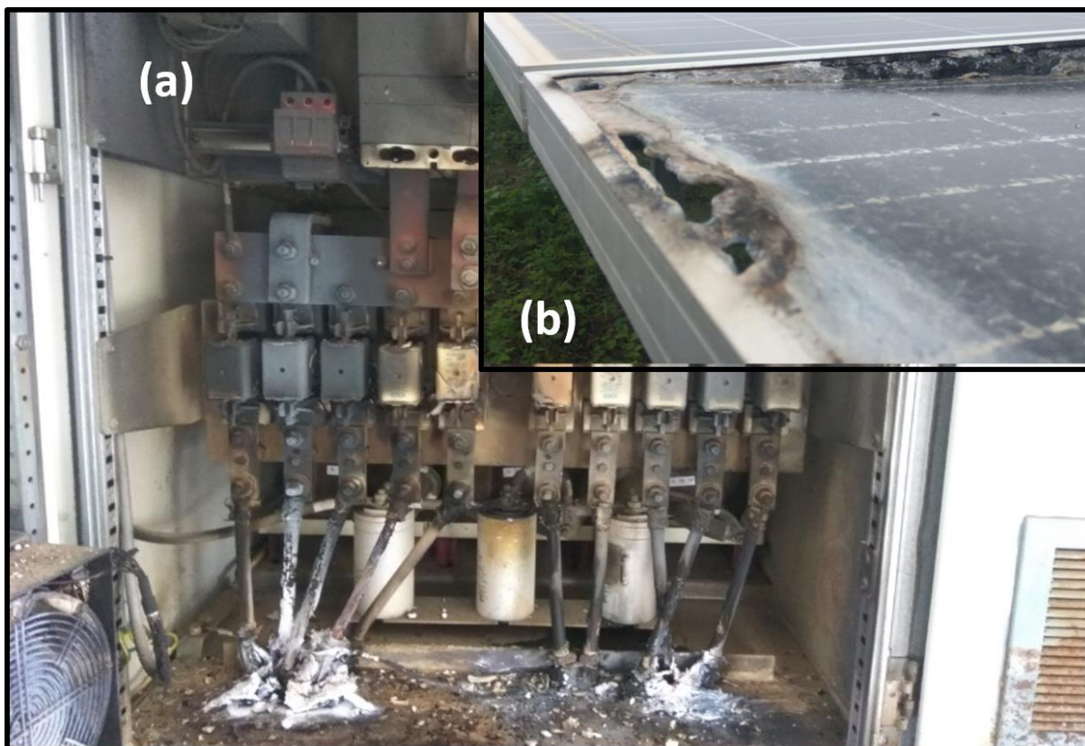
Figure 41: (a) Damaged SCB due to submergence. Prominent burn marks are seen. (b) Even though the modules were not submerged, severe burn marks that cause the melting of module glass were seen near module edges.
