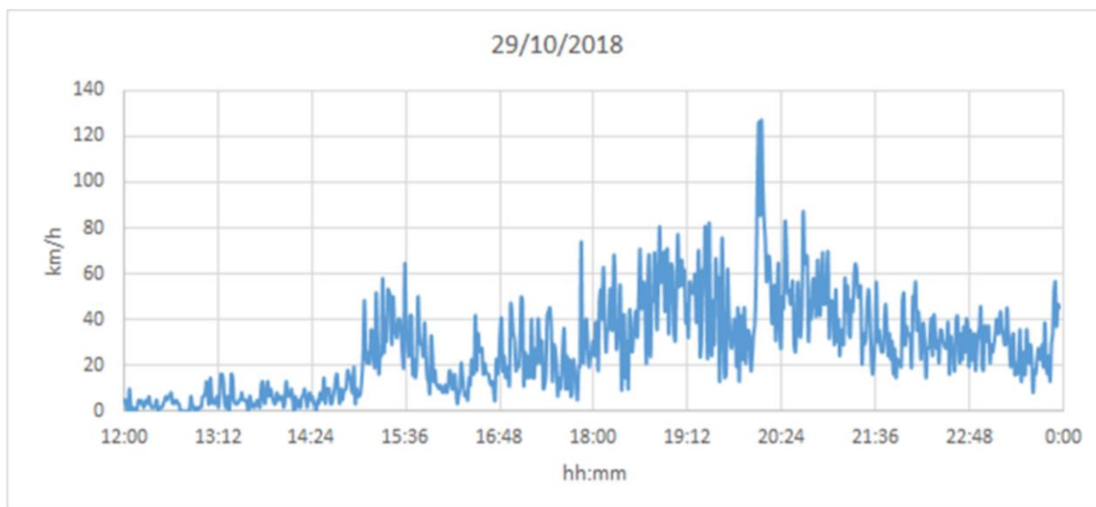
Figure 45: Gust speed during the windstorm day in Baselga di Piné, Italy. Source: Lorenzo Mercuri [125].
