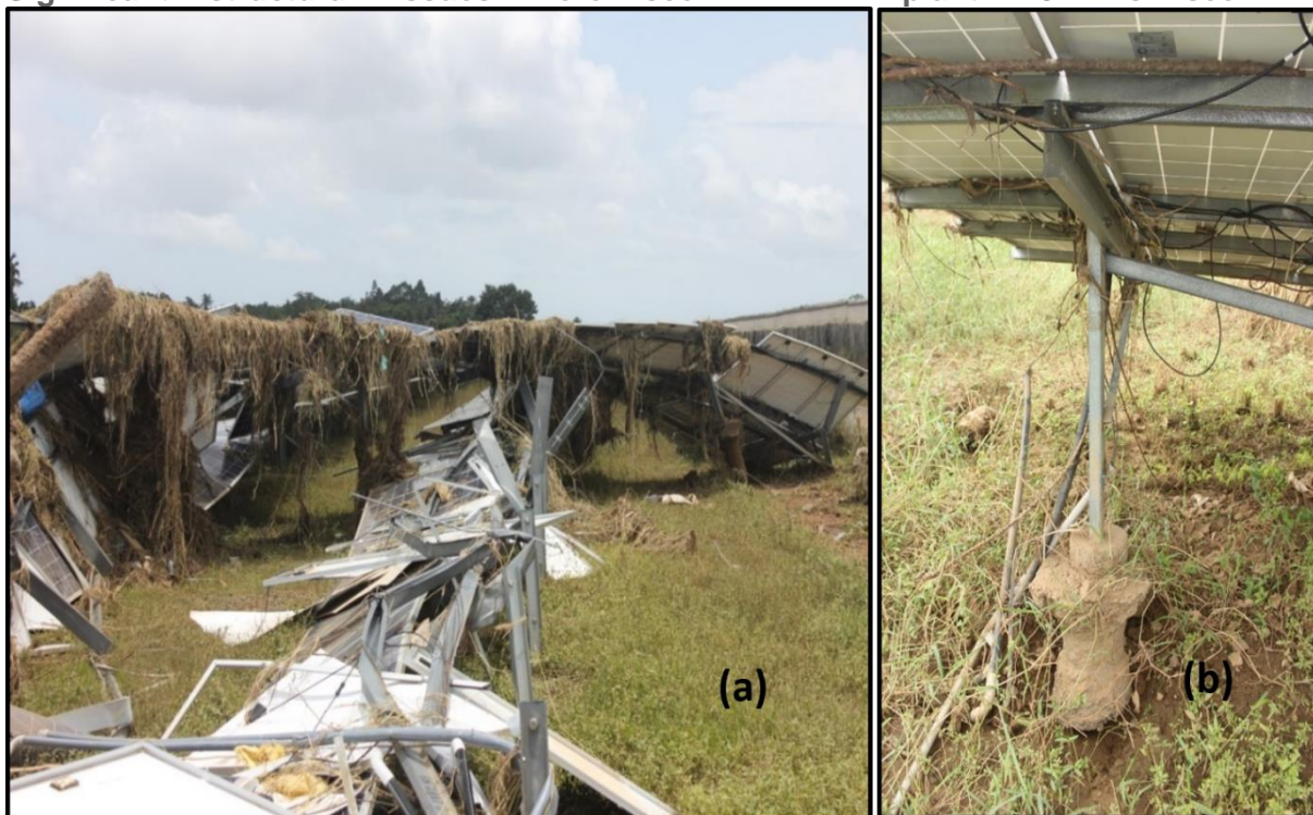
Figure 34 (a), the structures, module mounting clips, as well as modules were broken. In some cases, the laminates were seen to be separated from frames, wires detached from junction boxes, and broken glass was observed due to the impact of debris. In
