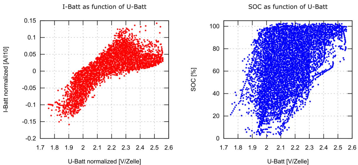
Figure 18: Battery current and SOC over normalized battery voltage
