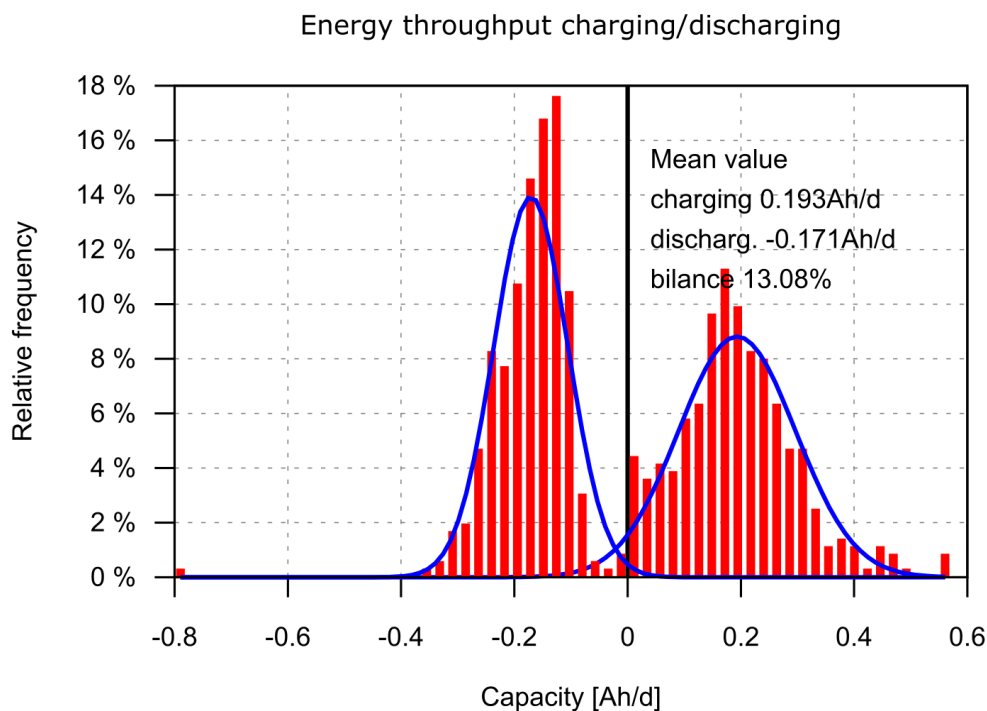
Figure 19: Frequency distribution of energy balance
