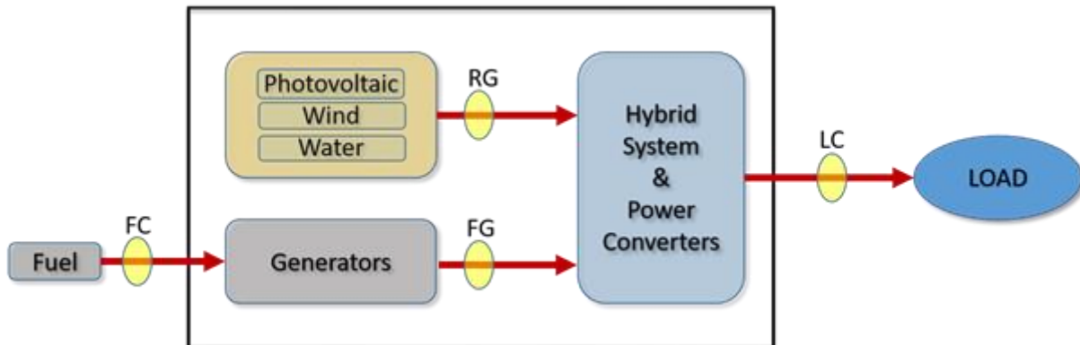
Figure 6: Schematic of measurement points for data analyses
