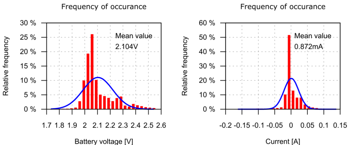
Figure 20: Frequency distribution of battery voltage and current
