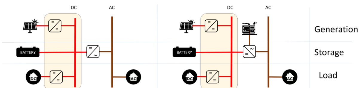
Figure 3: Schematic of an inverter system: left side is a pure inverter system and right side additionally with a backup generator
