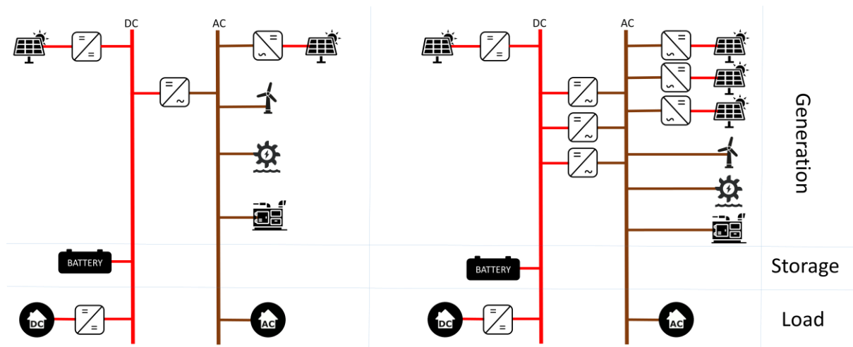
Figure 4: Single phase PV Hybrid System (left) and 3-phase PV Hybrid System (right)
