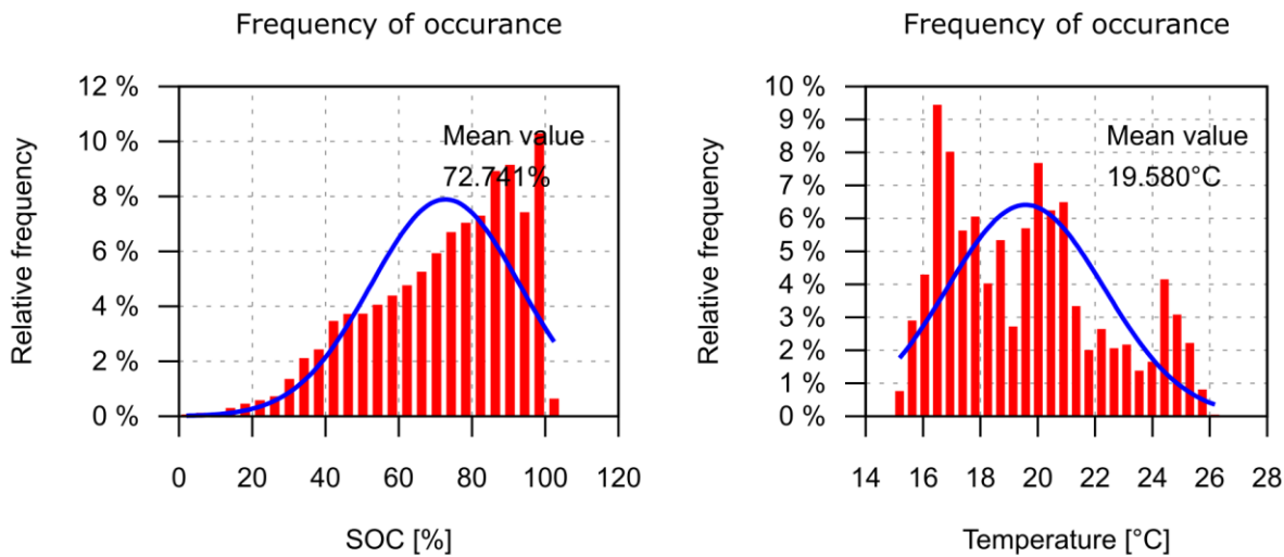
Figure 21: Frequency distribution of SOC and temperature
