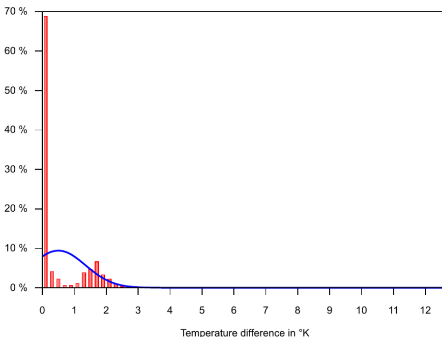
Figure 14: Histogram of temperature difference
