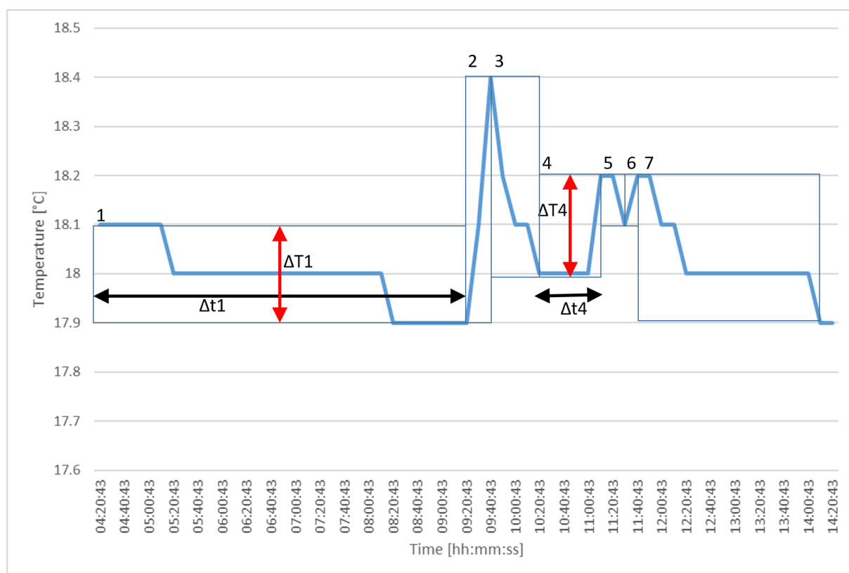
Figure 12: Calculating the parameter delta profile
